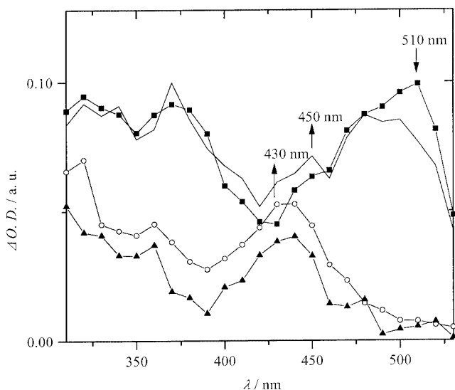
Figure 3. Transient spectra obtained upon LFP ( \lambda = 355 nm) of 3 ( 5 \times 10^{-4} M) in acetonitrile under argon, in the presence of 1a ( 1.2 \times 10^{-2} M); spectra recorded 0.4 μs (solid squares), 0.08 μs (straight line), 5 μs (open circles) and 8 μs (solid triangles) after the laser pulse
