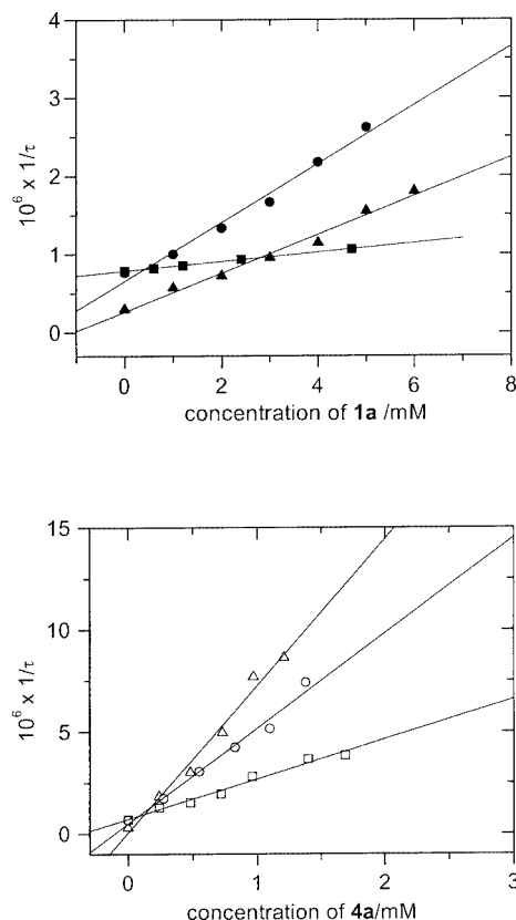
Figure 5. Plot to obtain k_q(T_1) for quenching of triplet 3 by 1a (top) and 4a (bottom) in several solvents: C_6H_6 (squares), MeCN (triangles) and MeOH (circles)
