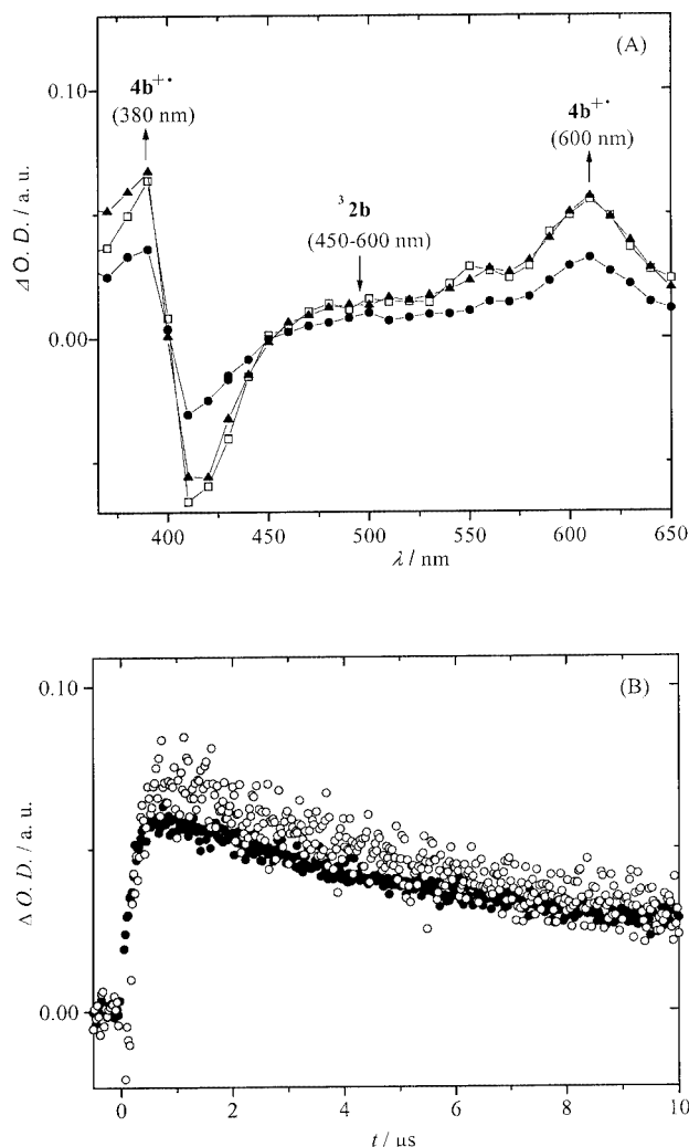
Figure 1. (A) Transient spectra obtained upon LFP ( \lambda = 355 nm) of 2b ( 0.75 \times 10^{-4} M) in acetonitrile under argon, in the presence of 1b ( 1.2 \times 10^{-3} M); spectra recorded 0.3 \mu s (open squares), 1 \mu s (solid triangles) and 5 \mu s (solid circles) after the laser pulse; (B) growth and decay of the 380-nm (open circles) and 600-nm (solid circles) bands
