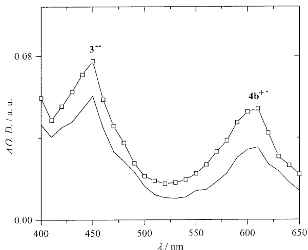
Figure 4. Transient spectra obtained upon LFP ( \lambda = 355 nm) of 3 ( 5 \times 10^{-4} M) in acetonitrile under argon, in the presence of 1b ( 2.9 \times 10^{-3} M), spectra recorded 0.3 μs (open squares) and 1 μs (line) after the laser pulse
