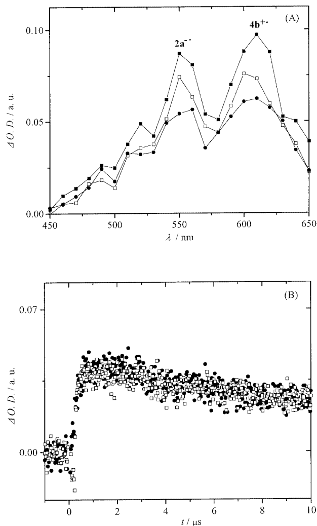
Figure 2. (A) Transient spectra obtained upon LFP ( \lambda = 355 nm) of 2a ( 1.25 \times 10^{-4} M) in acetonitrile under argon, in the presence of 1b ( 6.25 \times 10^{-4} M); spectra recorded 1 \mu s (solid squares), 3 \mu s (open squares) and 6 \mu s (solid circles) after the laser pulse; (B) growth and decay of the 550-nm (open squares) and 600-nm (solid circles) bands
