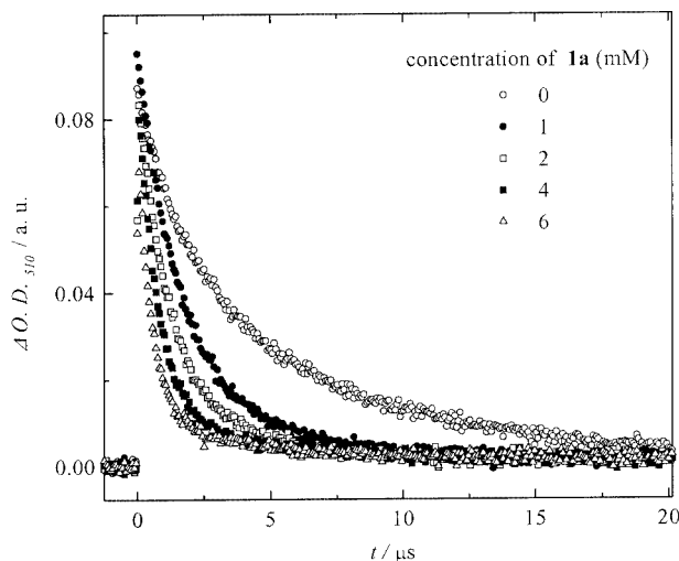
Figure 5. Decay traces of the T–T absorption of 3 ( 10^{-3} M) measured at 510 nm in the presence of increasing amounts of 1a , using acetonitrile as solvent
